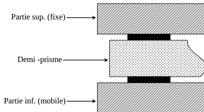
Figure 4.4 : Essai de compression simple.
