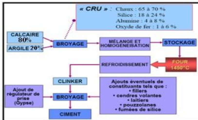
Figure 3.5: Etapes de fabrication du ciment portland.
